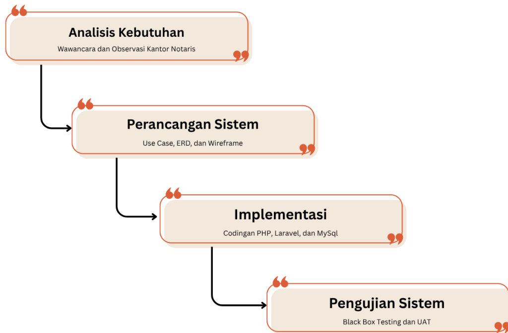
Gambar 1.1 Metode Waterfall
